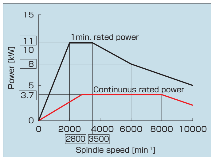
Standard spindle
