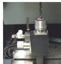
Tool length switch for automatic measurement
